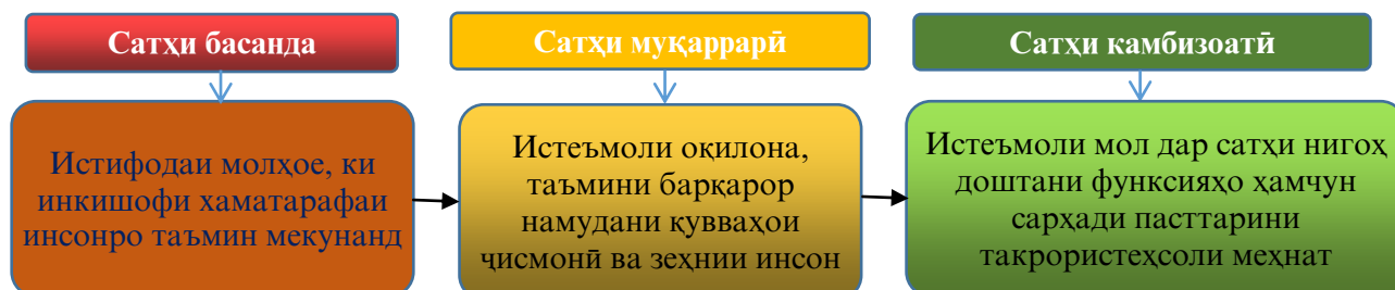
Figure 2. The structure of the classification of the quality of life of the population
